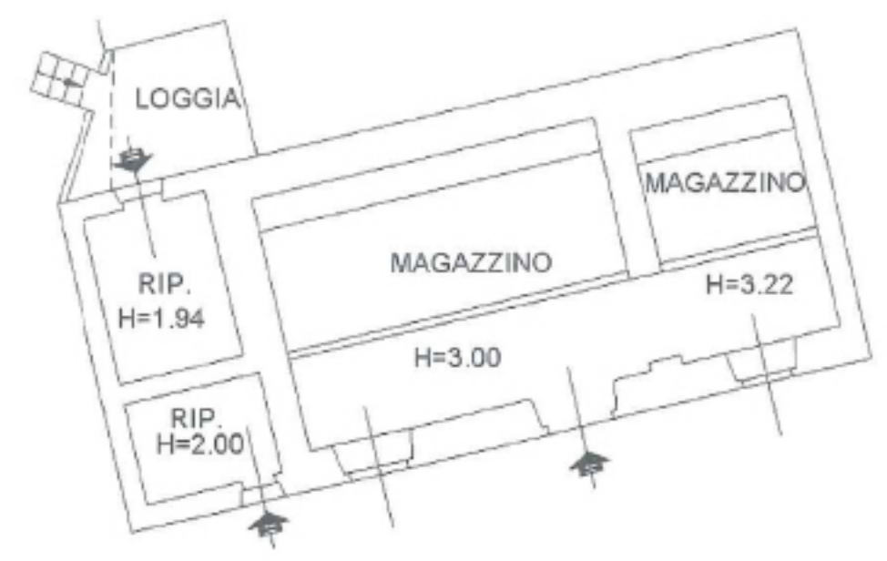
PIANO SEMINTERRATO
