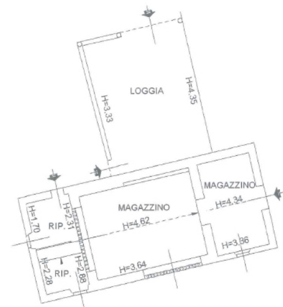
PIANO TERRENO
